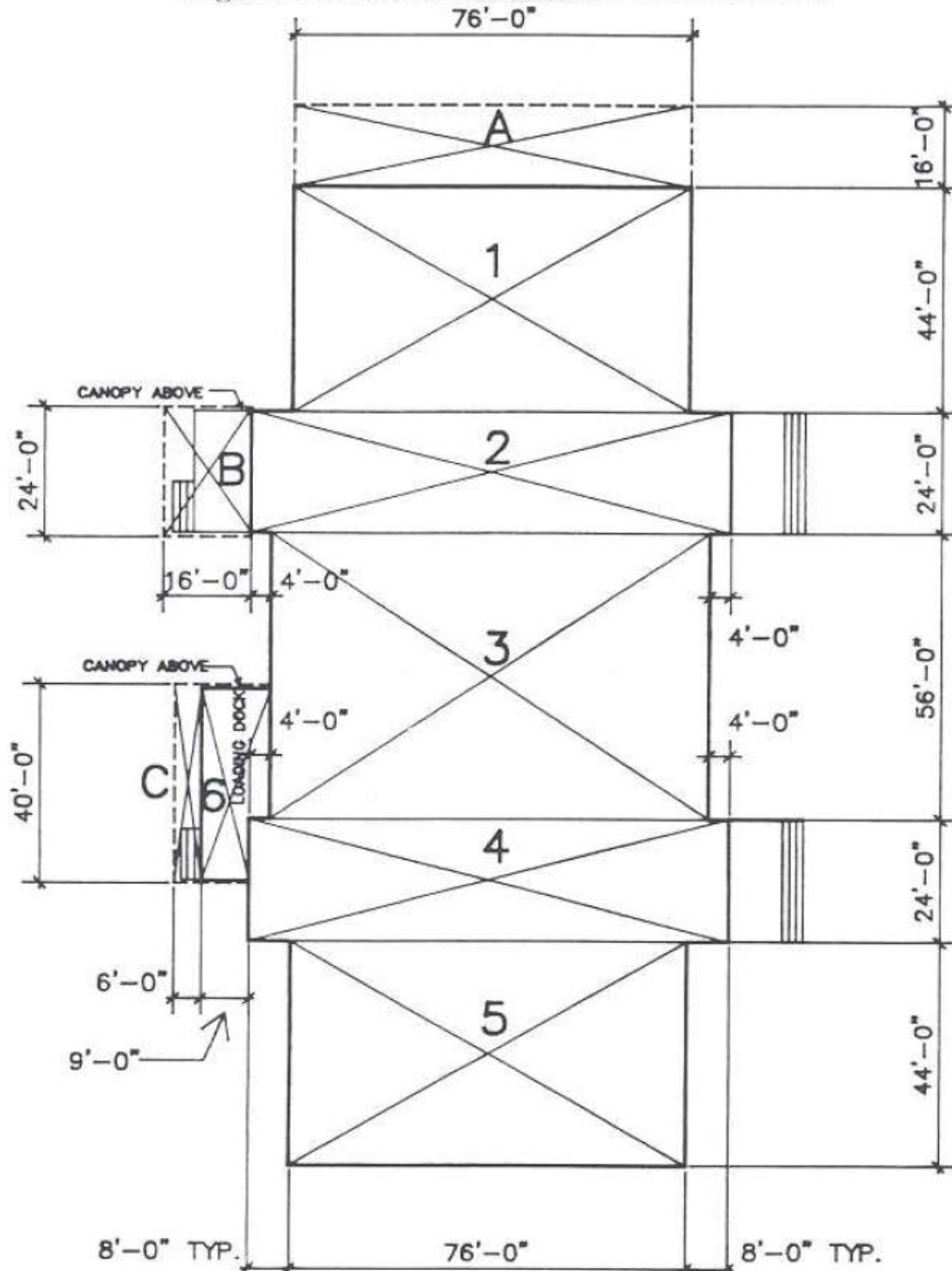
Figure 7. DIAGRAM OF BUILDING AREAS
