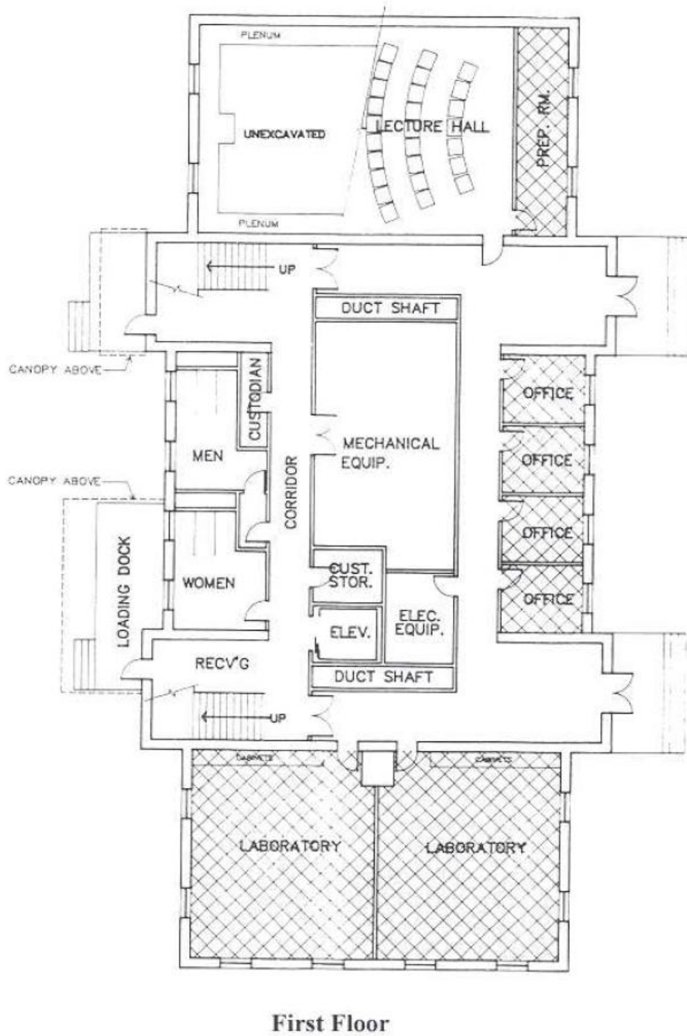
Figure 2A. Assignable Area
