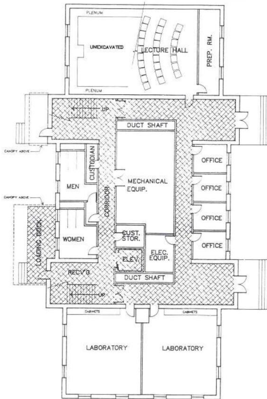
Figure 3A. Non-Assignable Areas: Circulation Area
